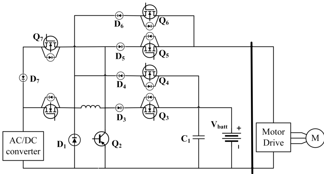
Figure 55. Integrated bidirectional AC/DC-DC/DC converter [33].
