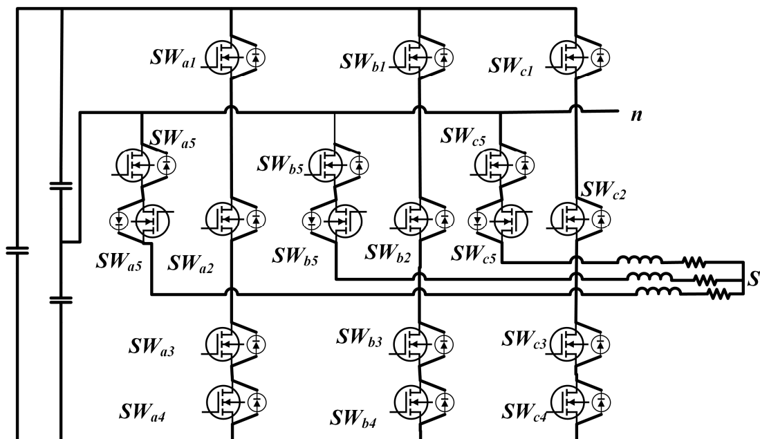
Figure 44. Novel stacked matrix inverter as shown in [97].
