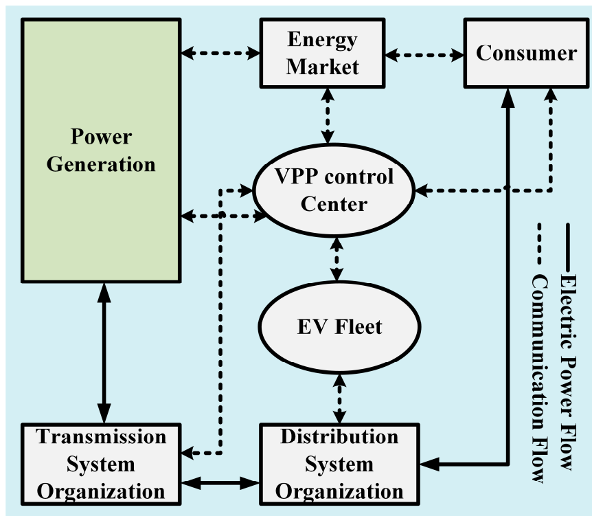
Figure 62. VPP architecture and control [117].
