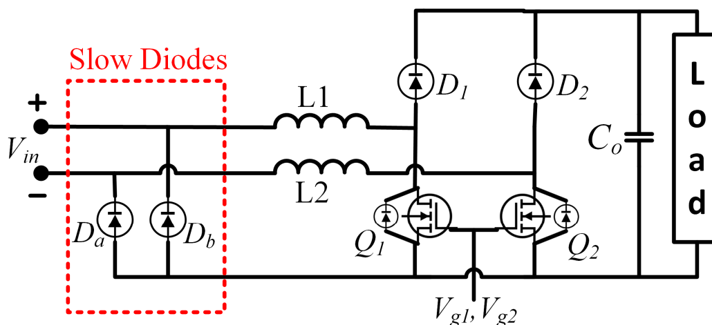
Figure 46. Bridgeless/Dual Boost PFC Converter. Adapted from [46].
