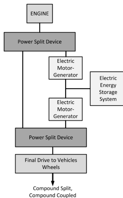
Figure 24. Compound split e-CVT system. Adapted from [32].
