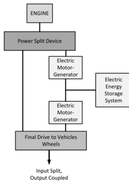
Figure 23. Input split e-CVT system. Adapted from [32].
