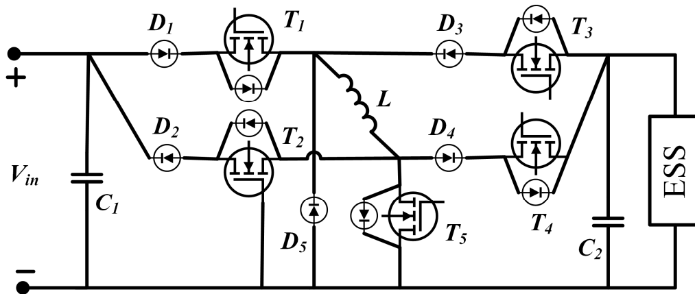
Figure 41. Universal DC-DC converter [72].
