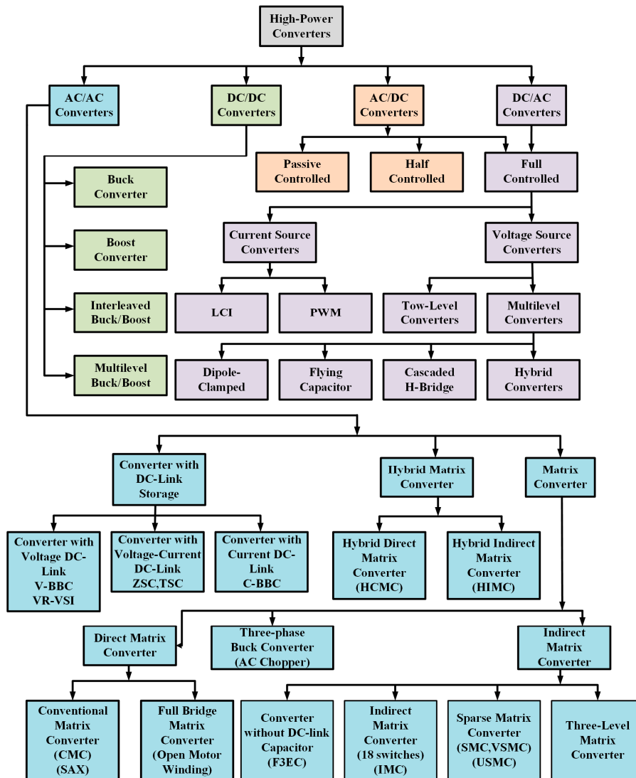
Figure 40. Detailed classification of converters. Data from [92,93].
