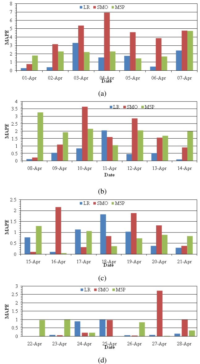
FIGURE 1: Daily MAPE of LR, SMO regression and M5P techniques to compare forecast accuracy of daily cases for the first wave of COVID-19 in the USA for the duration— (a) 01-07 April, 2020 (b) 08-14 April, 2020 (c) 15-21 April, 2020 (d) 22-28 April, 2020.
