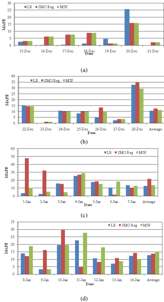
FIGURE 12: Daily MAPE of LR, SMO regression and M5P techniques to compare forecast accuracy of daily cases for the third wave of COVID-19 in India for the duration—(a) 15-21 Dec, 2021 (b) 22-28 Dec, 2021 (c) 01-07 Jan, 2022 (d) 08-14 Jan, 2022.
