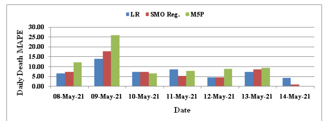
FIGURE 11: Daily MAPE for the duration 08-14 May, 2021 of LR, SMO regression and M5P techniques to compare the accuracy of daily death forecast for the second wave of COVID-19 in India
