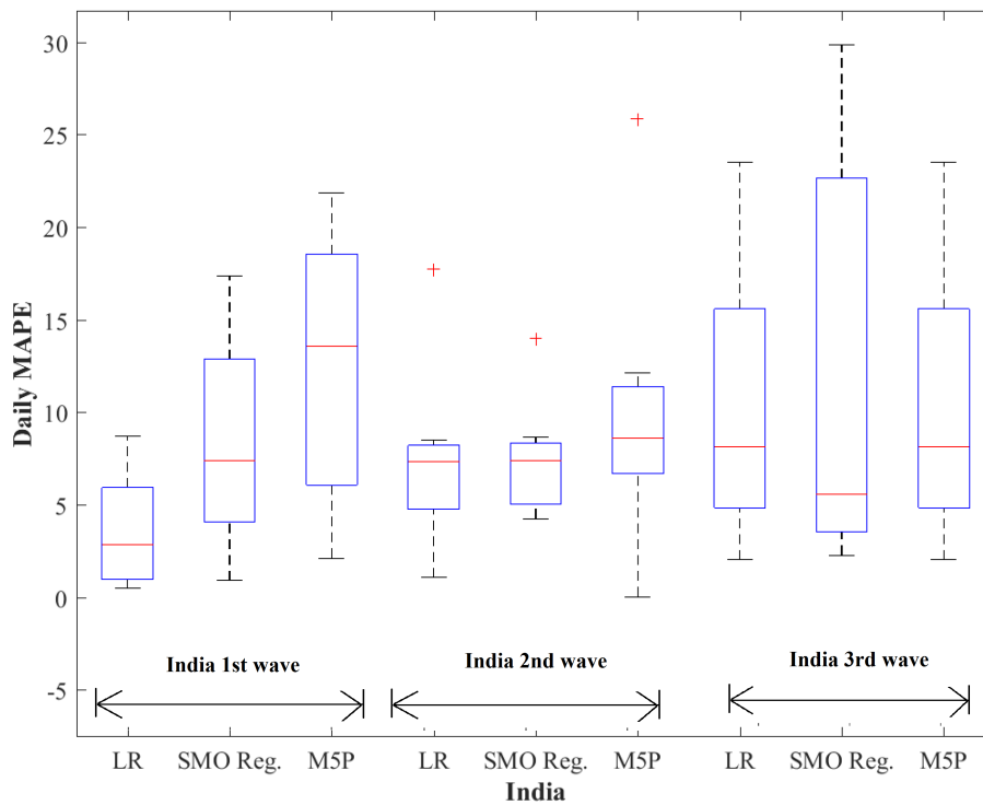
FIGURE 16: Box plot of Daily MAPE of India during First, Second and Third wave
