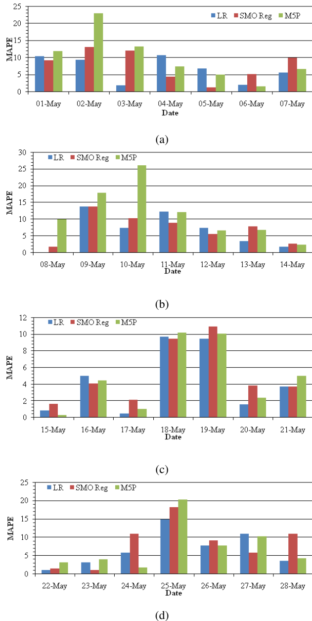
FIGURE 9: Daily MAPE of LR, SMO regression and M5P techniques to compare forecast accuracy of daily cases for the second wave of COVID-19 in India for the duration—(a) 01-07 May, 2021 (b) 08-14 May, 2021 (c) 15-21 May, 2021 (d) 22-28 May, 2021.
