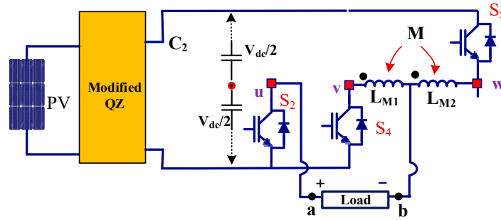
Figure 15. During mode-6 the inverter switches S 2 , S 4 , and S 5 are turned ON.
