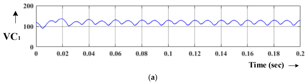
Figure 34. Inverter DC-link voltage at T_{ST} = 20\% .
