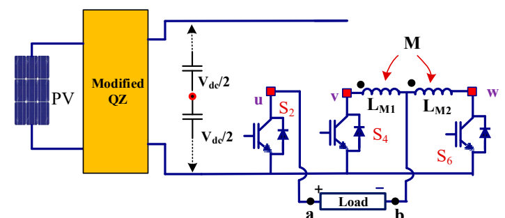
Figure 14. During mode 5 the inverter switches S_2 , S_4 , and S_6 are turned ON.
