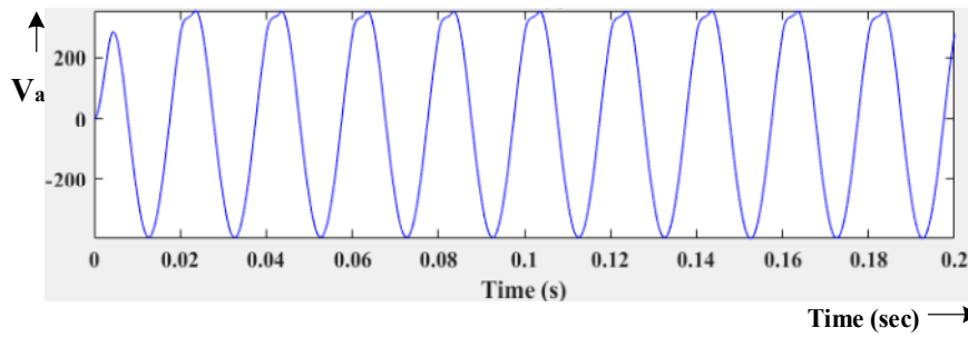
Figure 31. Inverter output current at T_{ST} = 25\% with filter.
