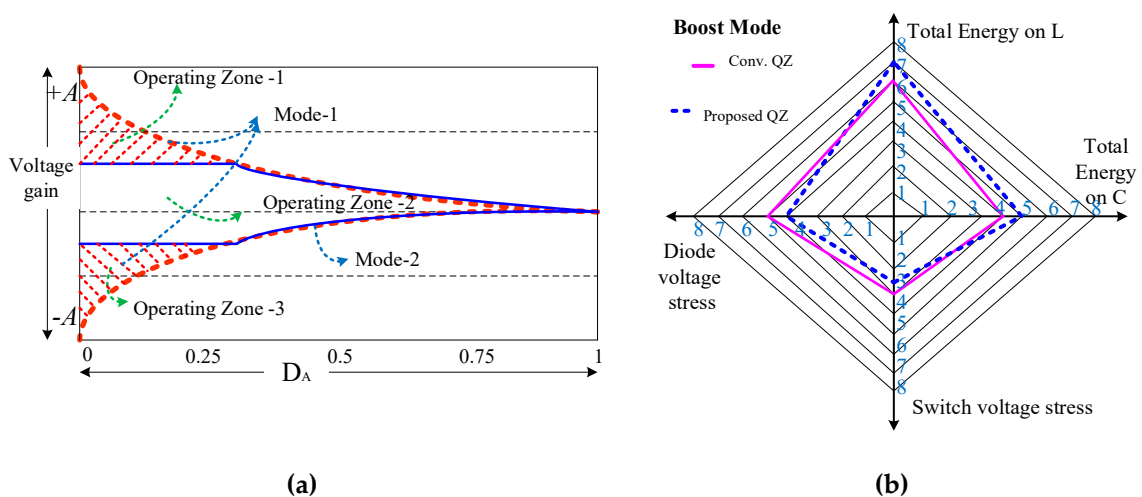
Figure 8. (a) Converter operation in different modes, V_{boost} / input voltage ( V_{PV} ) for duty cycle D_A , (b) energy storage capability and voltage stress radar graph of conventional QZ and proposed QZ.
