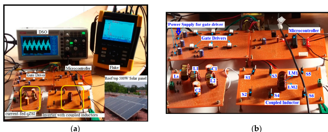
Figure 40. Experimental setup; (a) overall laboratory-scale 500 W PV powered modified Q-impedance fed coupled inductor MLI, (b) modified Q-impedance fed coupled inductor MLI.
