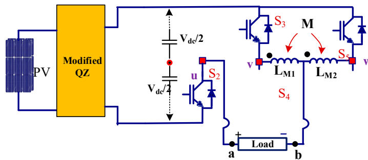
Figure 17. During Mode-8 the inverter switches S 2 , S 3 , and S 5 are turned ON.
