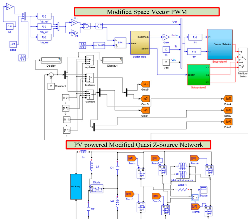
Figure 23. Simulation diagram of the proposed photovoltaic (PV) powered modified Q-impedance converter fed coupled inductor MLI.
