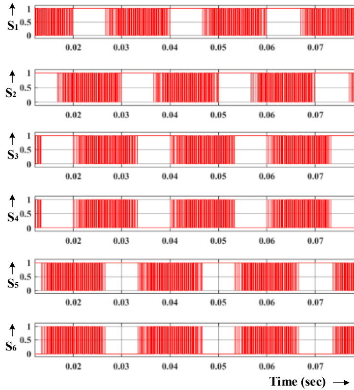
Figure 24. Modified Q-impedance converter fed coupled inductor MLI.
