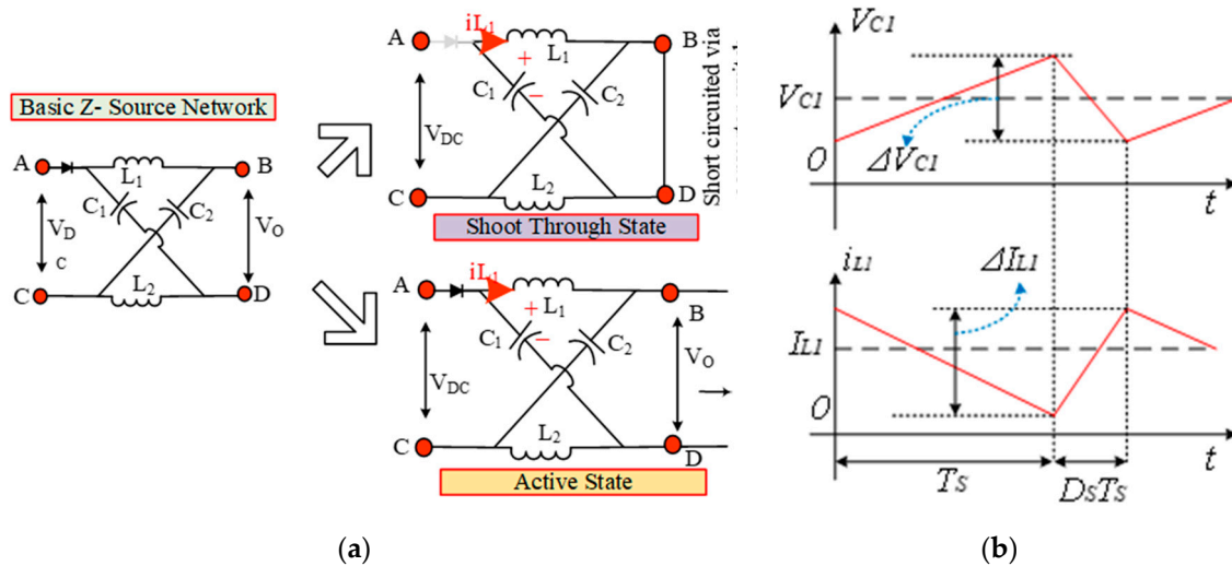
Figure 2. Impedance source inverter operation: (a) impedance source circuit, shoot through (ST) state, an active state, (b) inductor current and capacitor voltage idealized condition waveforms.
