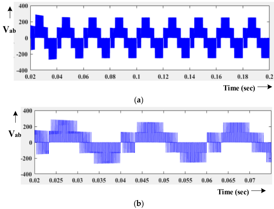
Figure 36. (a) Inverter output voltage at T_{ST} = 25\% without filter, (b) zoomed view of inverter output voltage at T_{ST} = 25\% without filter.
