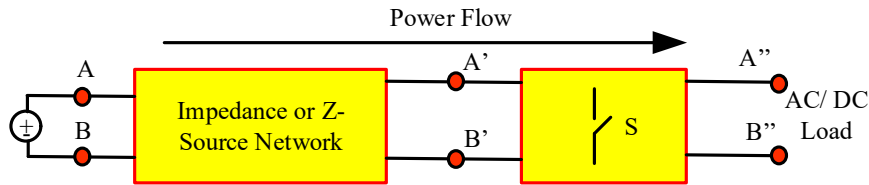
Figure 1. Impedance source inverter basic block diagram.
