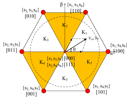
Figure 20. Space vector diagram and switching table.
