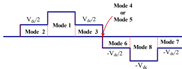
Figure 18. Output voltage structure for proposed MLI.
