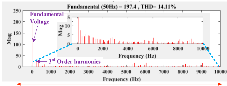
Figure 37. THD profile of inverter output voltage at T_{ST} = 25\% without a filter.
