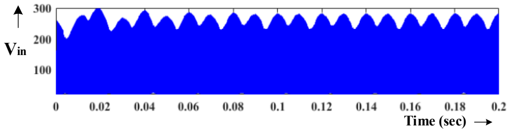
Figure 34. Inverter DC-link voltage at T_{ST} = 20\% .
