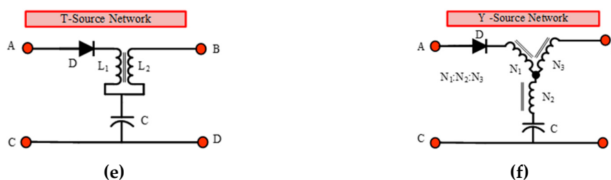
Figure 4. Different Z-source topologies; (a) Z-source network, (b) Quasi-source network, (c) Modified Quasi-source network, (d) Trans Z-source network, (e) T-source network, (f) Y-source network.
