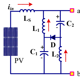
Figure 6. Proposed modified Q-impedance network.
