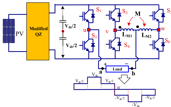
Figure 9. Coupled inductor MLI.
